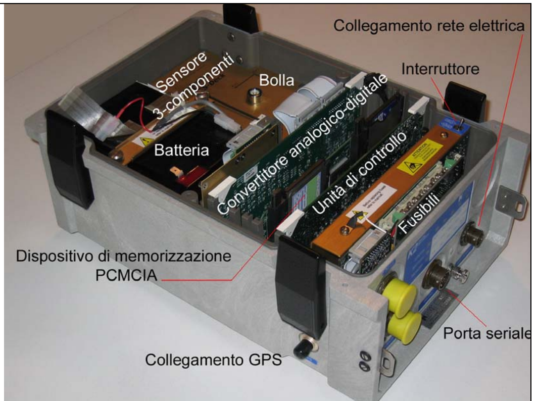
Figure 1– The digital accelerometer K2 with its main components.
