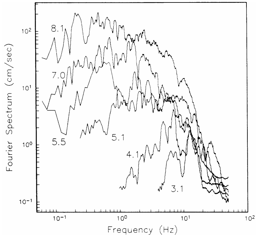
Figure 7 – Fourier Spectra of increasing magnitude accelerograms, recorded in 1985-1986 by digital instruments located on the Pacific coast of Mexico (Guerrero network)
